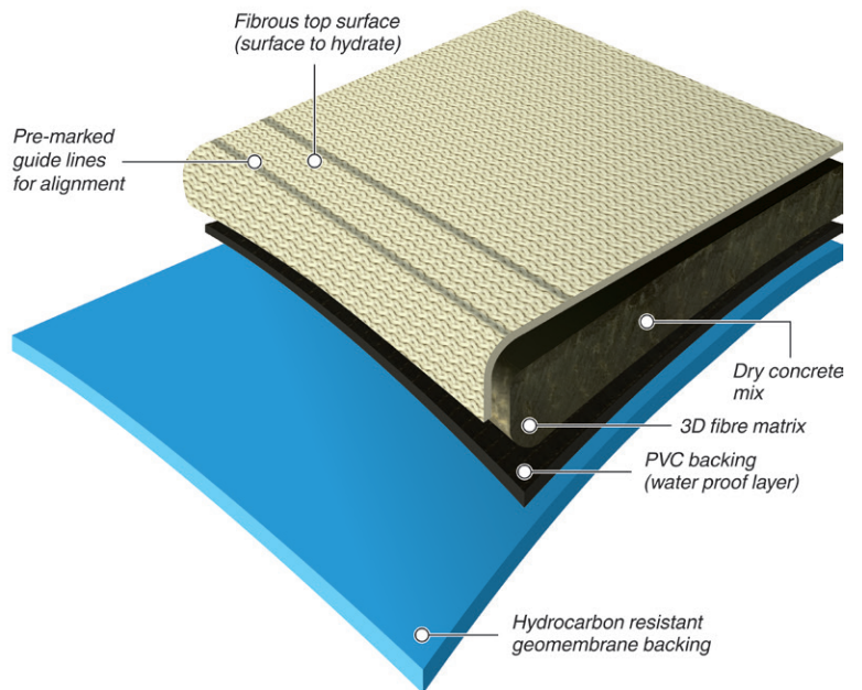
CC Hydro™ GCCB section
