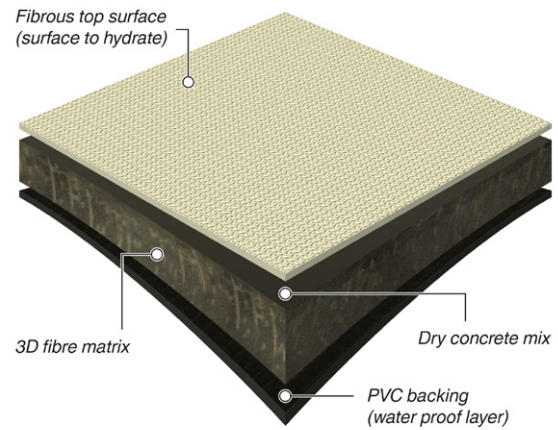
CC Hydro™ GCCB section
