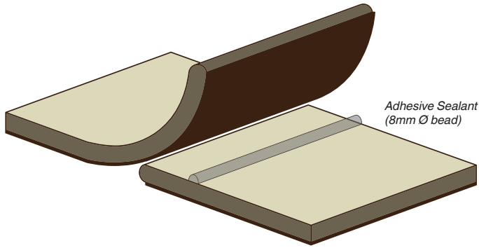
Adhesive sealant applied prior to screw jointing
